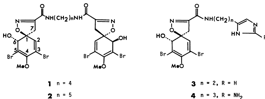
Fig. 1. Some novel spiroisoxazolines from marine sponges.
